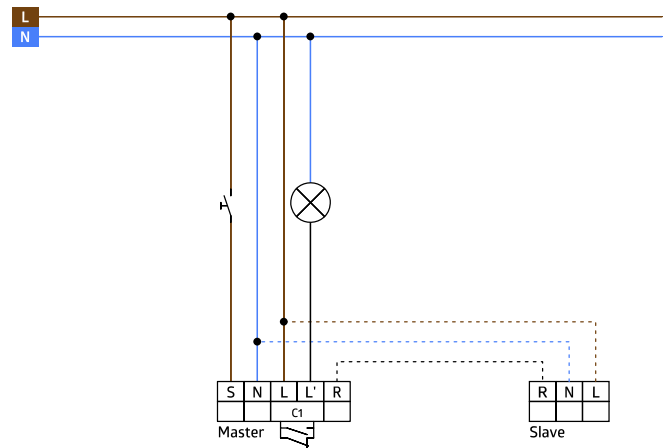
Wiring diagram
